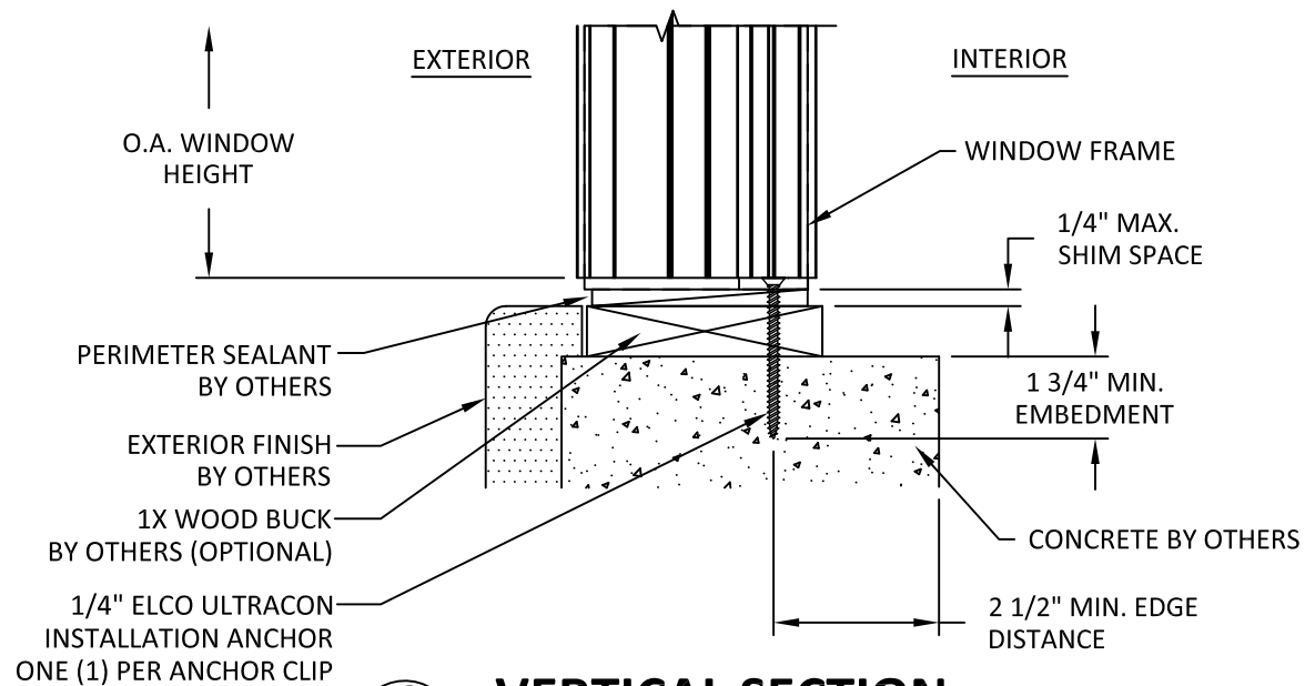
C 2 VERTICAL SECTION SILL - CONCRETE
