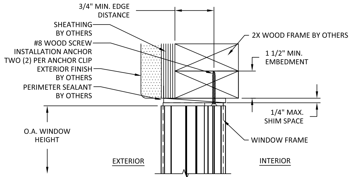
A 2 VERTICAL SECTION HEAD - 2X WOOD FRAME
